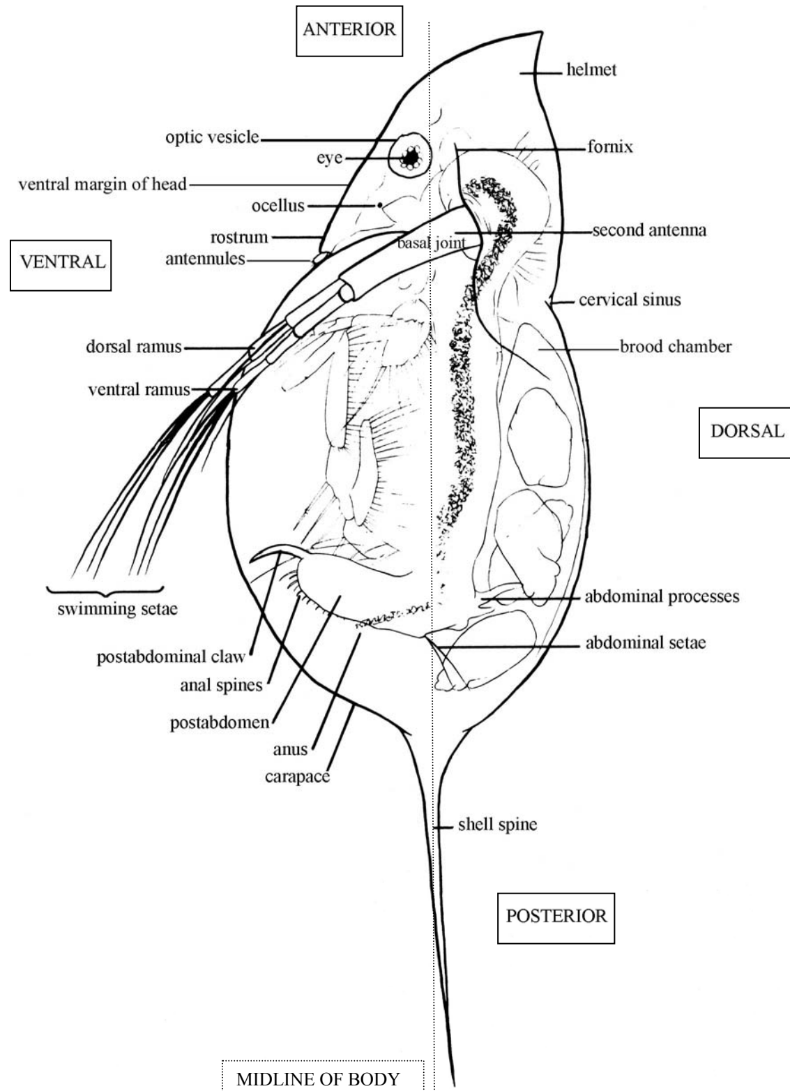
Figure 28. General anatomy of a daphnid (modified from Balcer et al., 1984)
