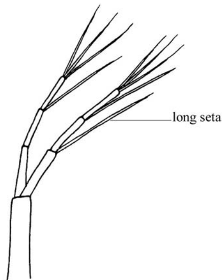
Figure 32. General depiction of a short vs. a long swimming seta on the 2 nd antenna (modified from Pennak, 1989)
