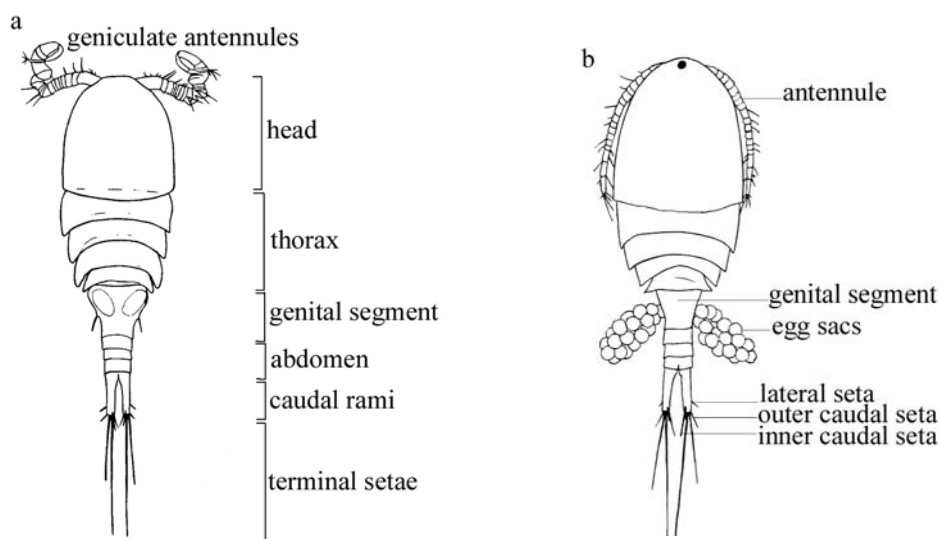
Figure 24. General anatomy of cyclopoid copepods showing key features in males (a) and females (b) (modified from Balcer et al., 1984)
