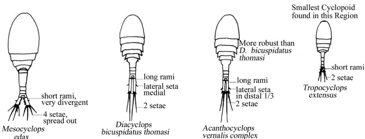
Figure 25. Comparative representations of common cyclopoid members (modified from Torke, 1974)
