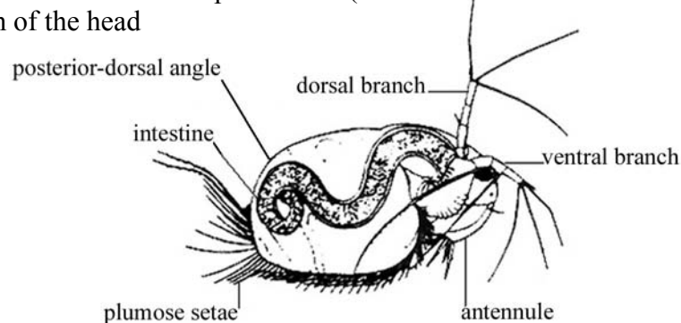
Figure 10. General diagram of a member of the family Macrothricidae (modified from Dodson and Frey, 1991)
